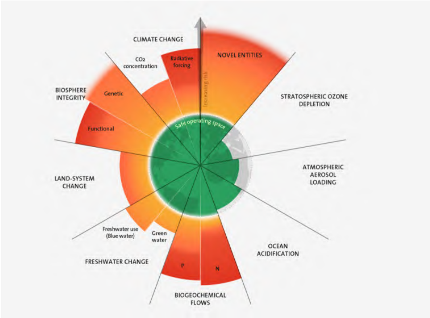
Graphic: Stockholmresilience.org Planetary Boundaries 2023 (9 Boundaries assessed, 6 crossed) 3
