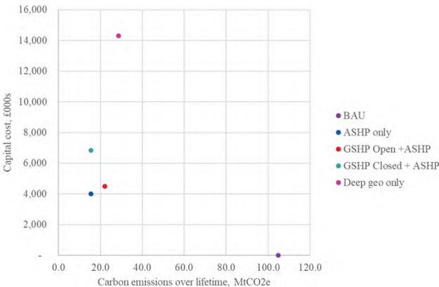
Figure 0.1: Techno-economic results summary with emissions
